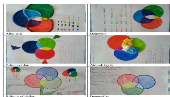
Figure 11. The Venn Diagrams Showing the Combination of Colors of Light
