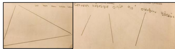
Figure 9. Examples of Forming a Right Triangle
