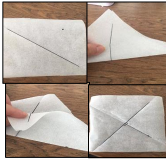
Figure 1. Finding the Shortest Distance of a Point from a Line
