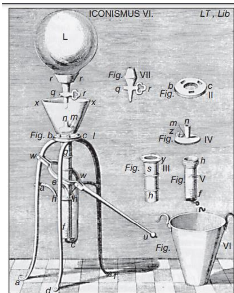
Picture: The air pump of Guericke (Jousten, 2016).
