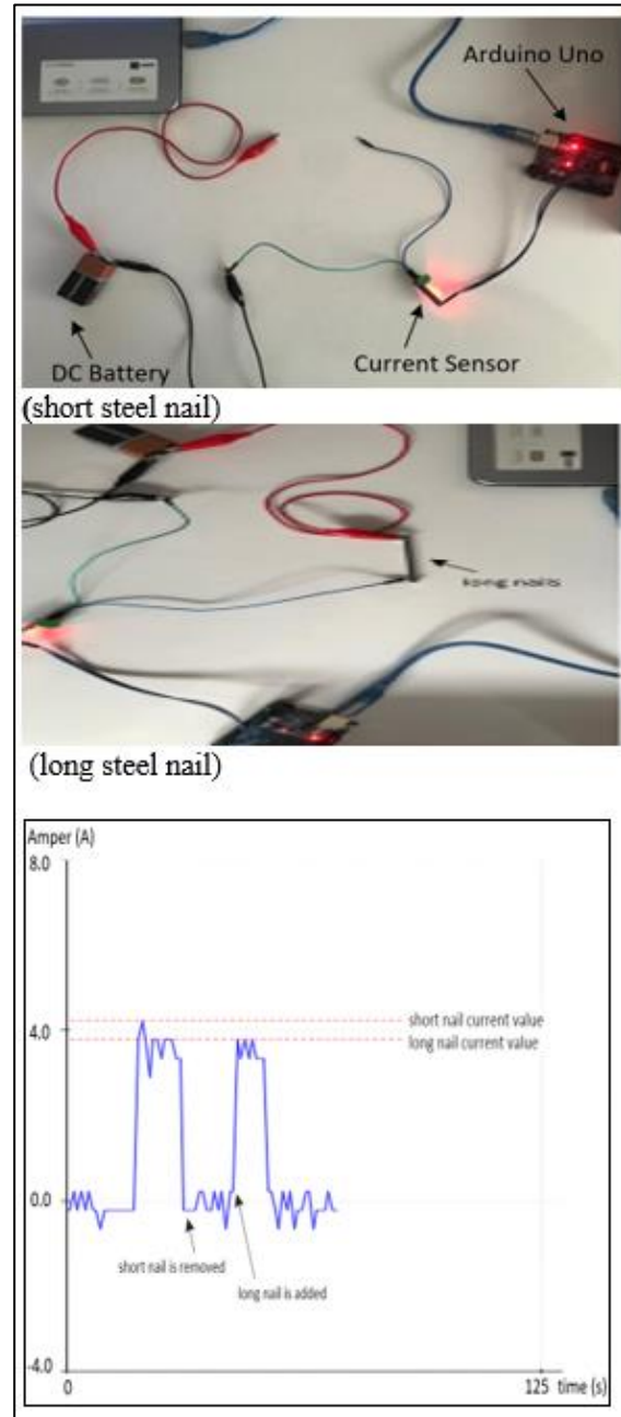
Figure 5. Experiment Setup for the Length of the Conductor and the Observation Made on the Serial Plotter
