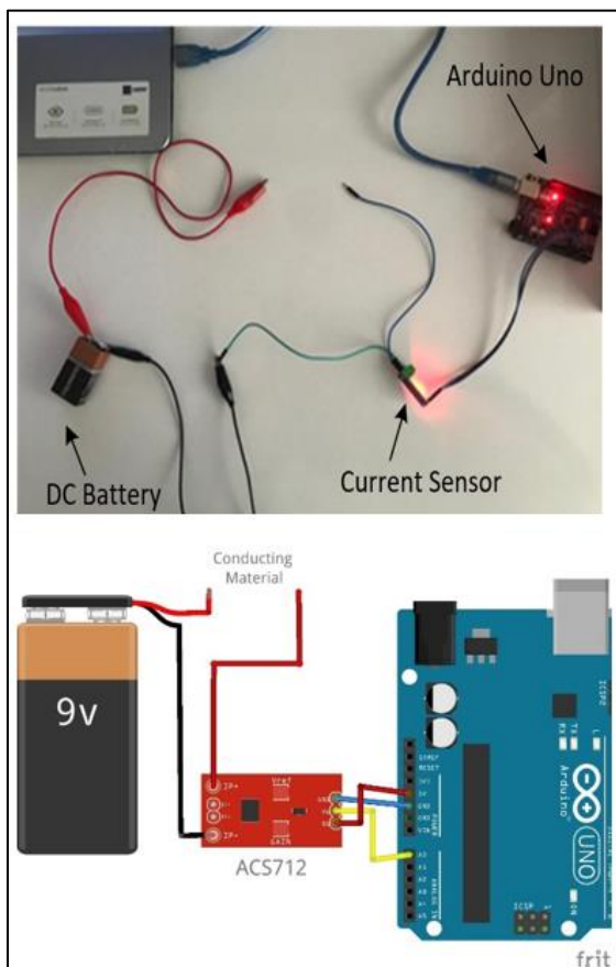
Figure 4. Robotic Setup Prepared and Its Diagram
