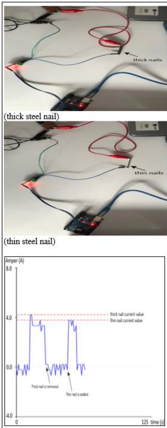
Figure 6. Experiment Setup for the Cross-sectional Area of the Conductor and the Observation Made on the Serial Plotter
