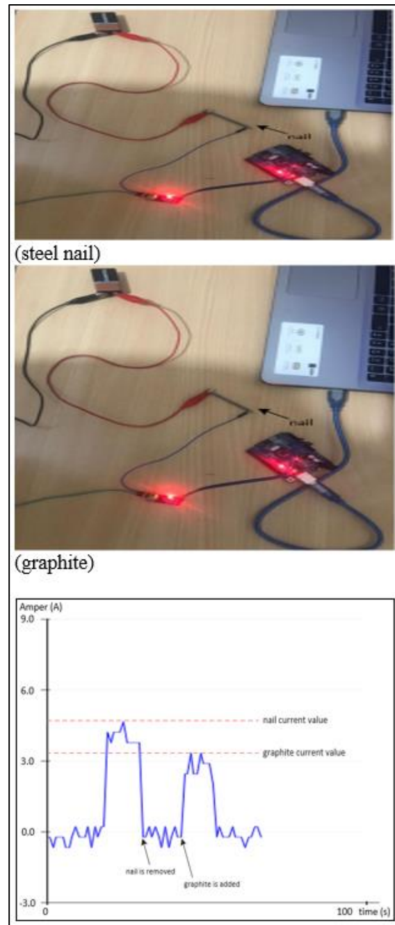
Figure 7. Experiment Setup for the Type of Conductor and the Observation Made on the Serial Plotter
