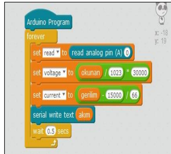
Figure 2. Ready-to-use Code Prepared Using mBlock
